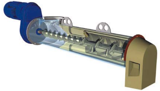
DELTA Silo type volumetric mixers
